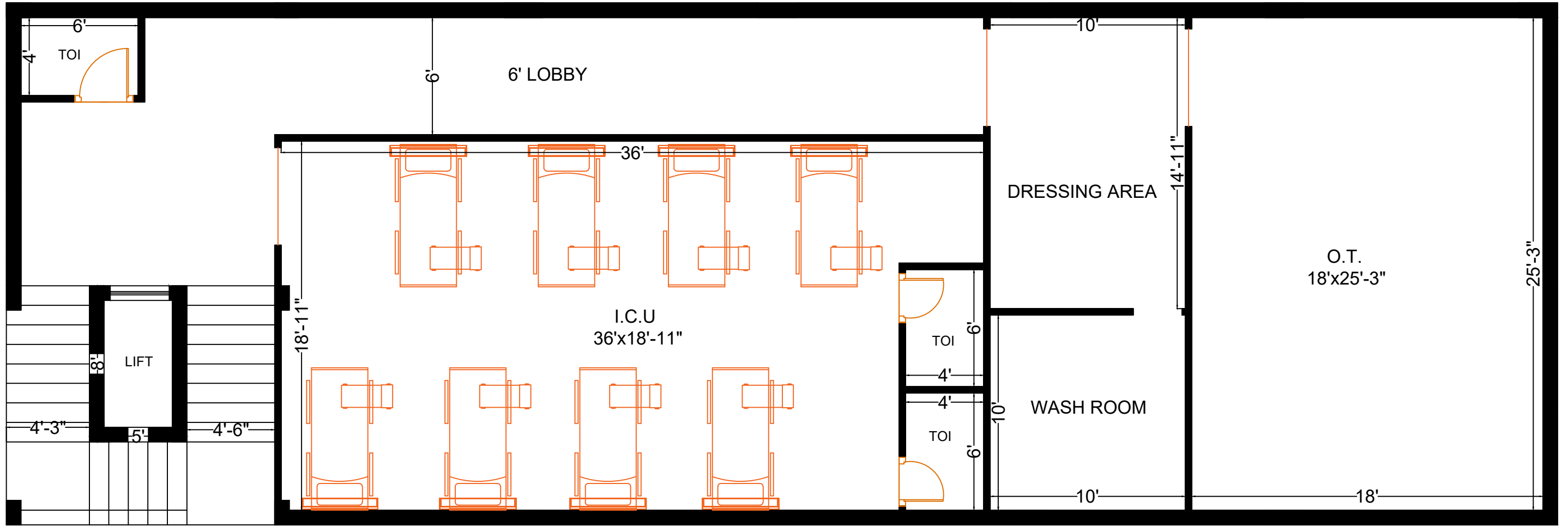
PRO-FIRST FLOOR PLAN
