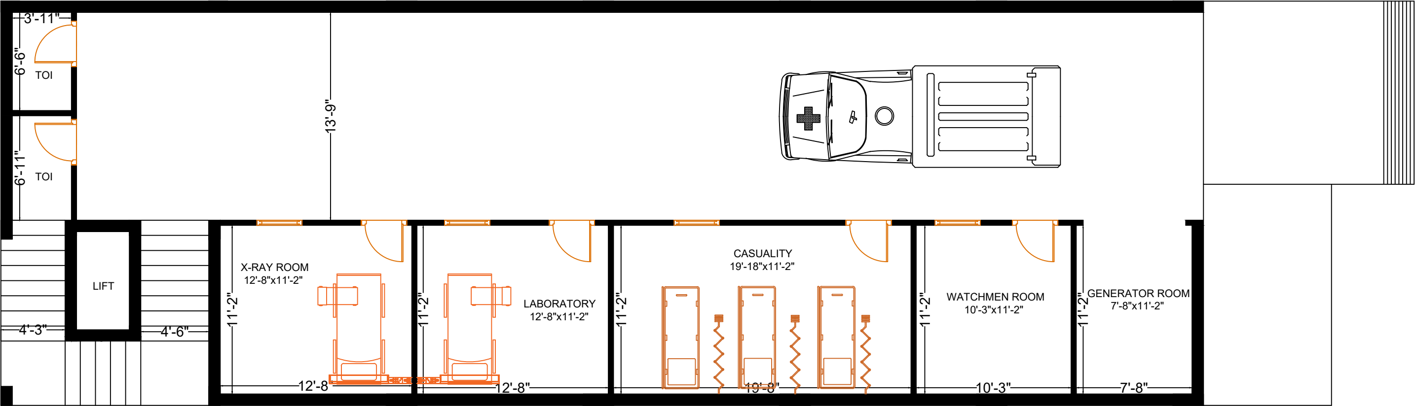
PRO-CELLAR PLAN
