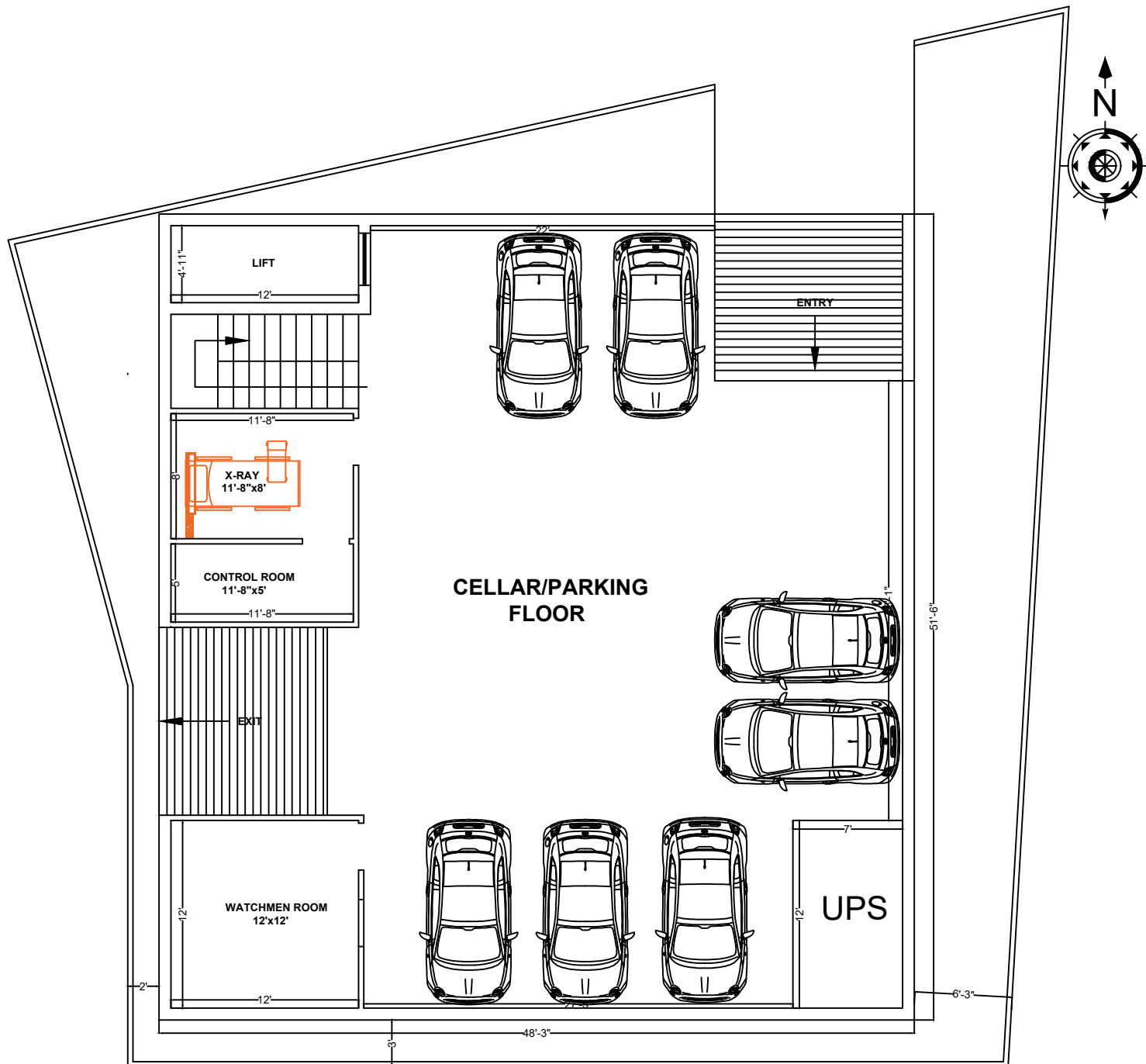
PRO-CELLAR FLOOR PLAN
