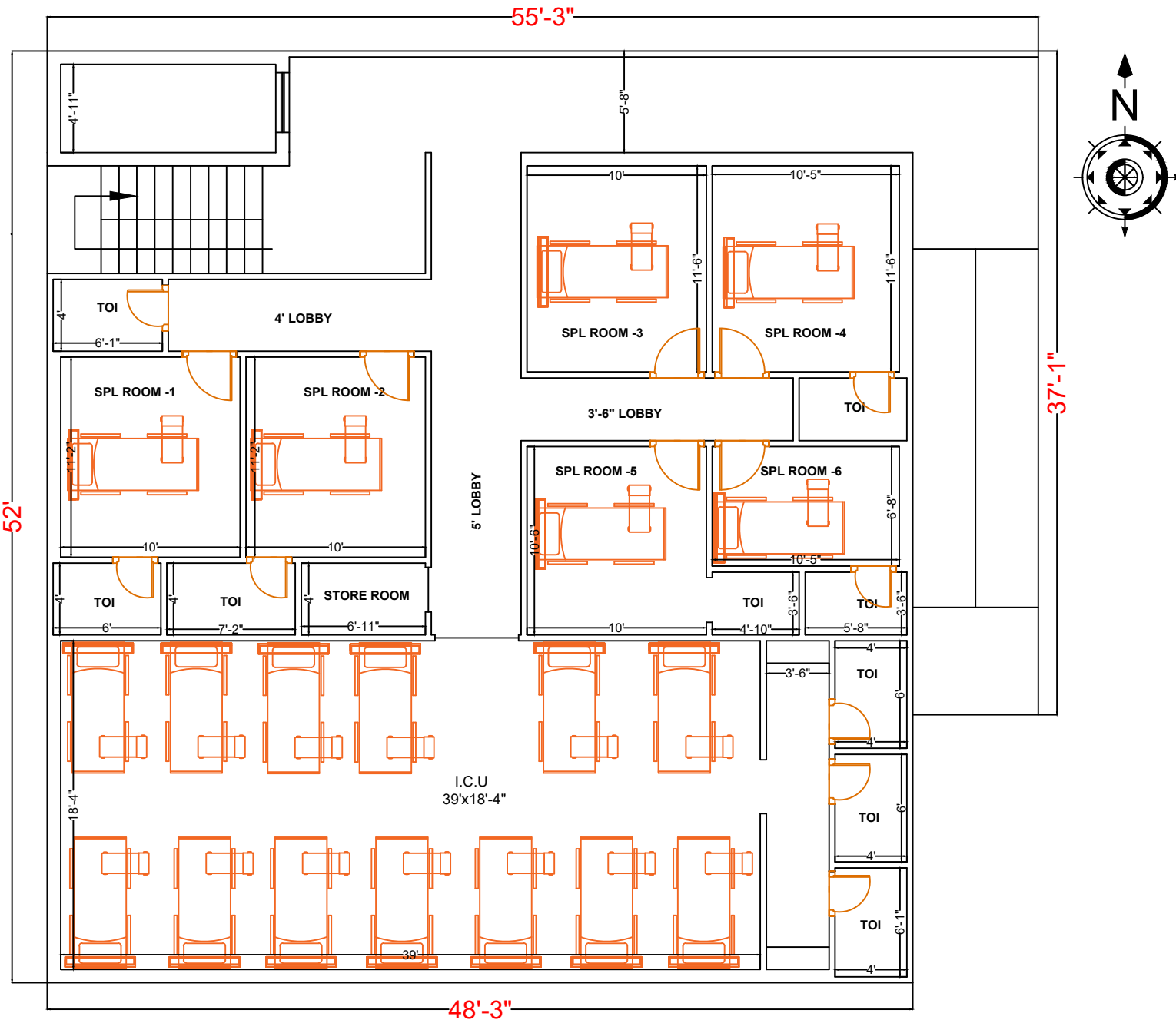
PRO-SECOND FLOOR PLAN
